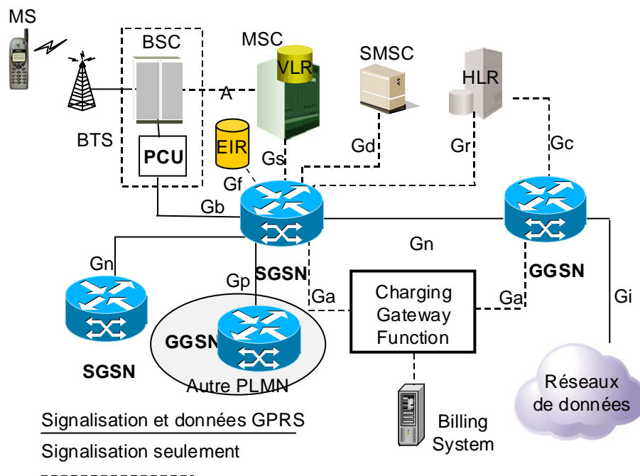
Figure 1 : Architecture GPRS
