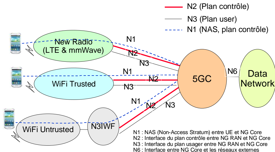
Figure 1 : Architecture 5GC
