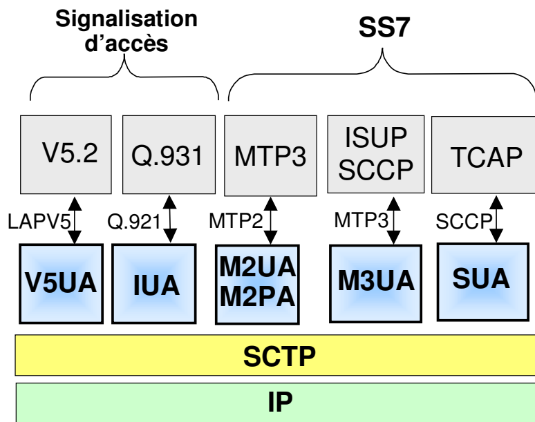
Figure 2 : Adaptations SIGTRAN
